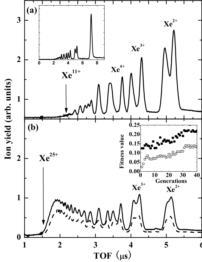
Figure 2.5: Time-of-flight (TOF) traces for the interaction of Xenon clusters ( N_{\text{avg}} \approx 1.6 \times 10^4 ) (a) with a Fourier-transform-limited 100\text{fs} , 800\text{nm} , 10^{15}\text{W}/\text{cm}^2 laser pulse (The inset shows the complete TOF trace); (b) with the best pulse found by a Genetic Algorithm in an 80-parameter unrestricted optimization (dashed line) and the best pulse found in a restricted 3-parameter optimization (solid line). The best pulse found by the GA consists of a sequence of two 120\text{fs} pulses, separated by 500\text{fs} . The inset in (b) shows the evolution of the fitness value for the 80-parameter optimization (full squares, maximum fitness; open squares, average fitness).
